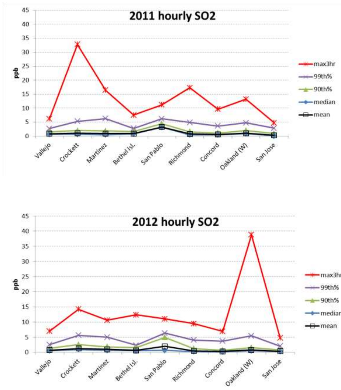
Figure 0-4. Annual statistics for SO 2 sites in the Bay Area. The primary NAAQS is 75ppb (99 th percentile) and secondary is 500 ppb (maximum 3hr average).
