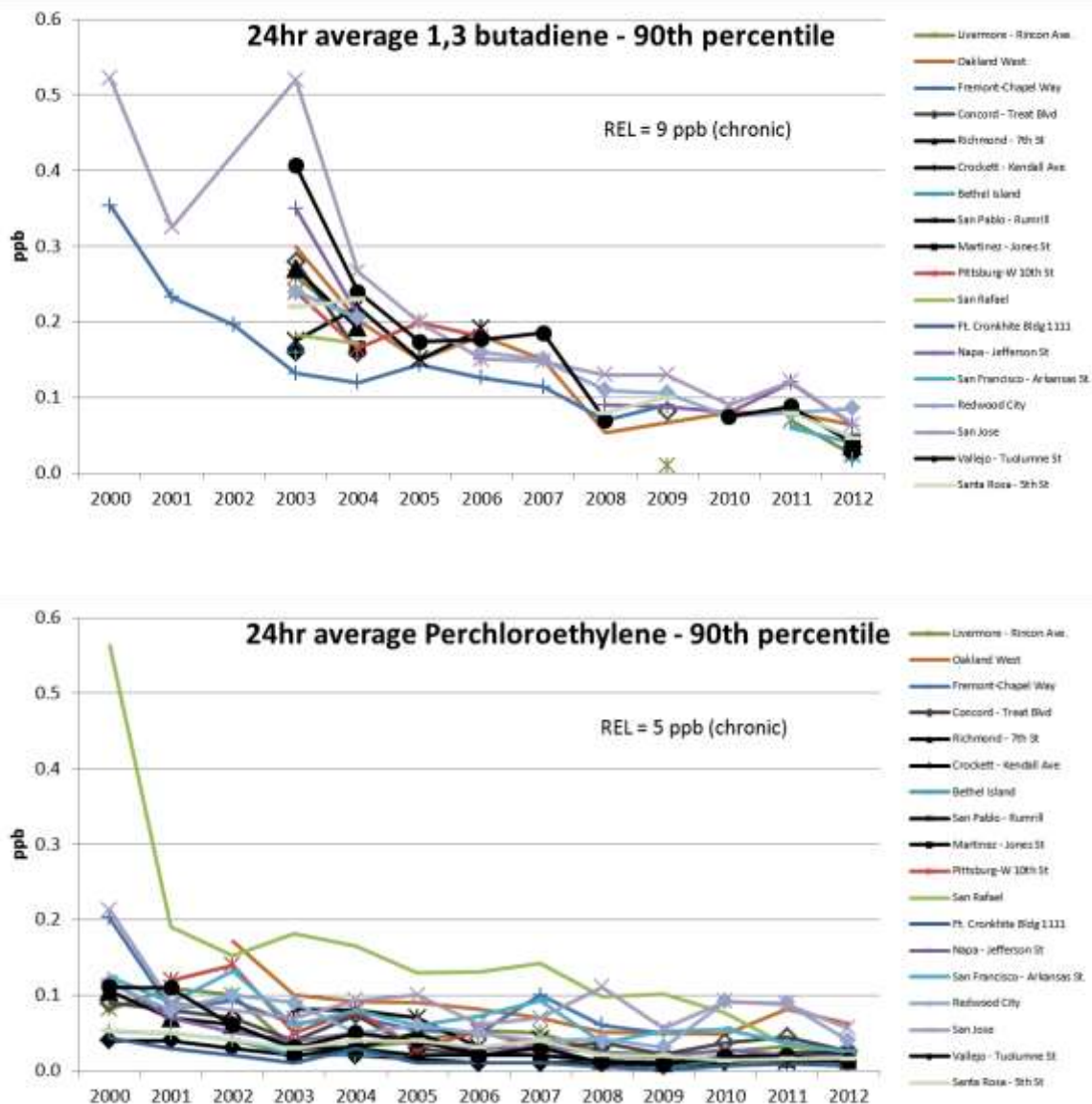
Figure 0-6. Trends in air toxics, 2000 – 2012. Sites near refineries are indicated by bold black lines. Values below LOD are not shown.
