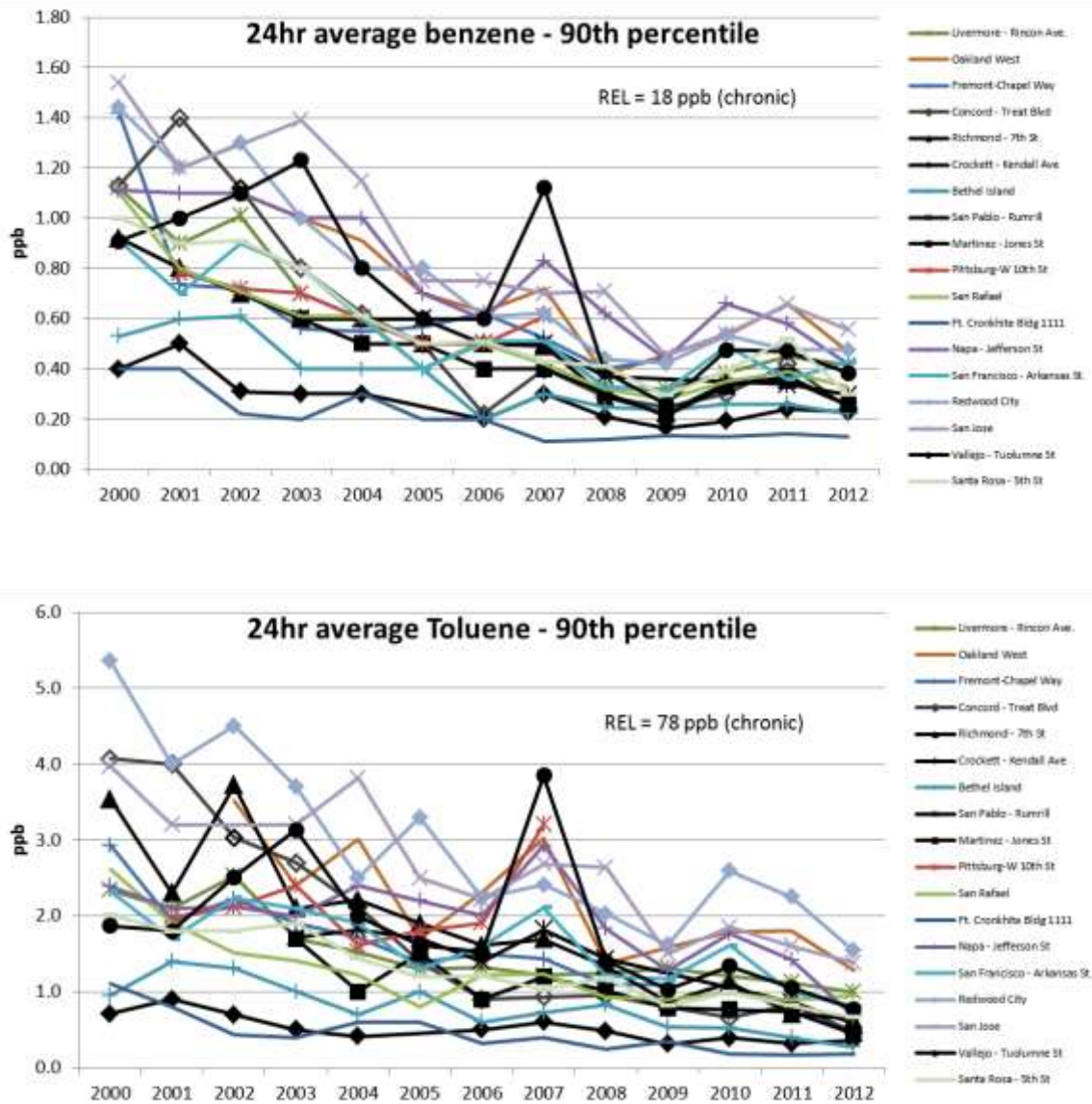
Figure 0-5. Trends in air toxics, 2000 – 2012. Sites near refineries are indicated by bold black lines. Values below LOD are not shown.
